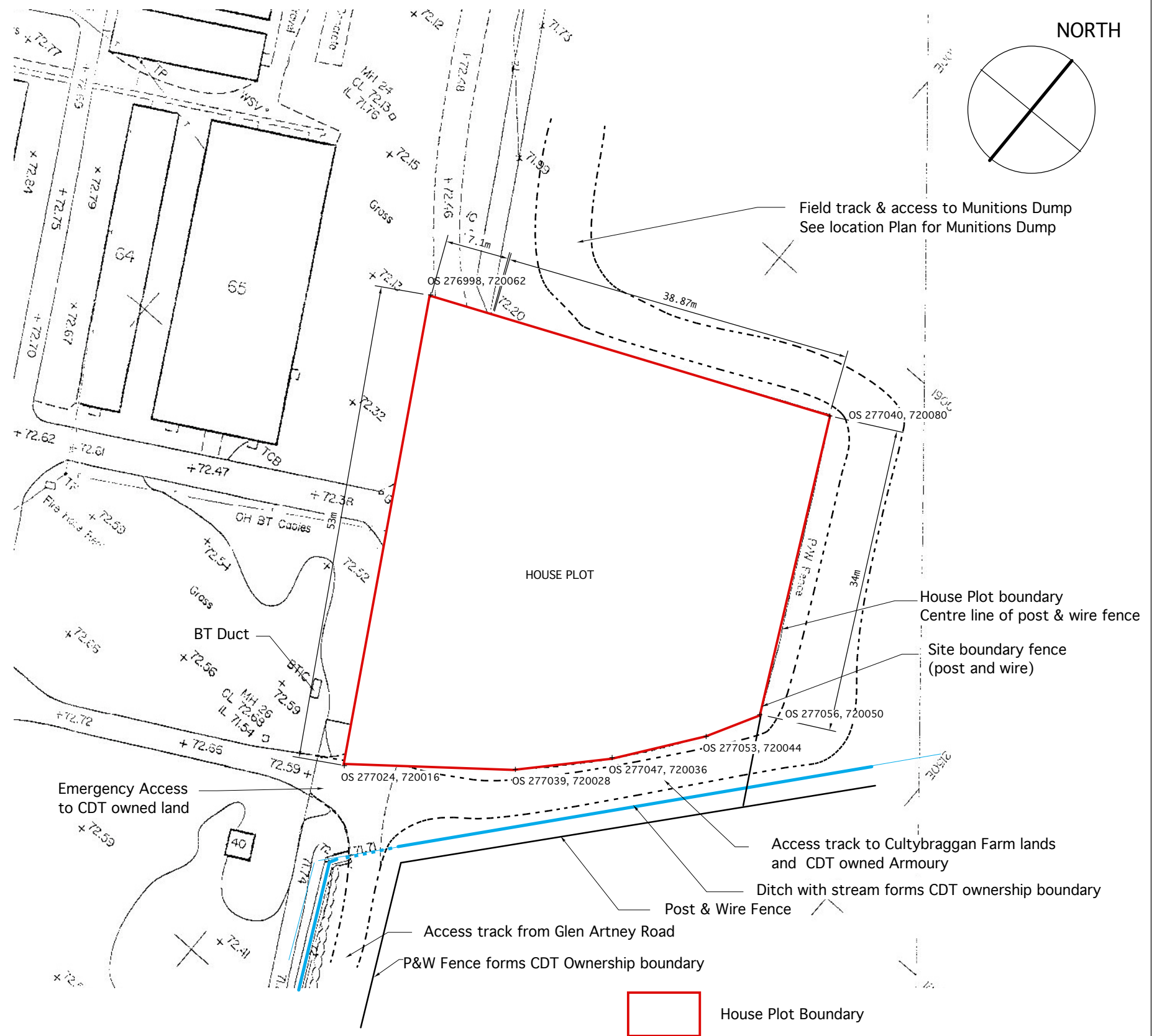
Plot Boundary Layout 1:250 Based on 1995 Mason Land Surveys Topographic Survey
